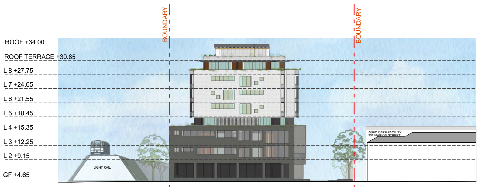
SOUTH ELEVATION
